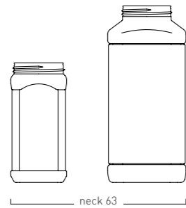
neck 63
