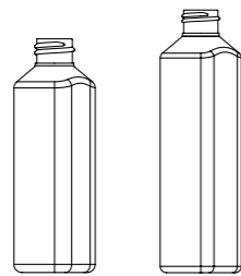
neck 20
