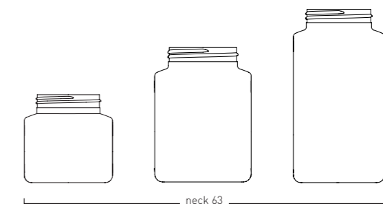
390 ml
